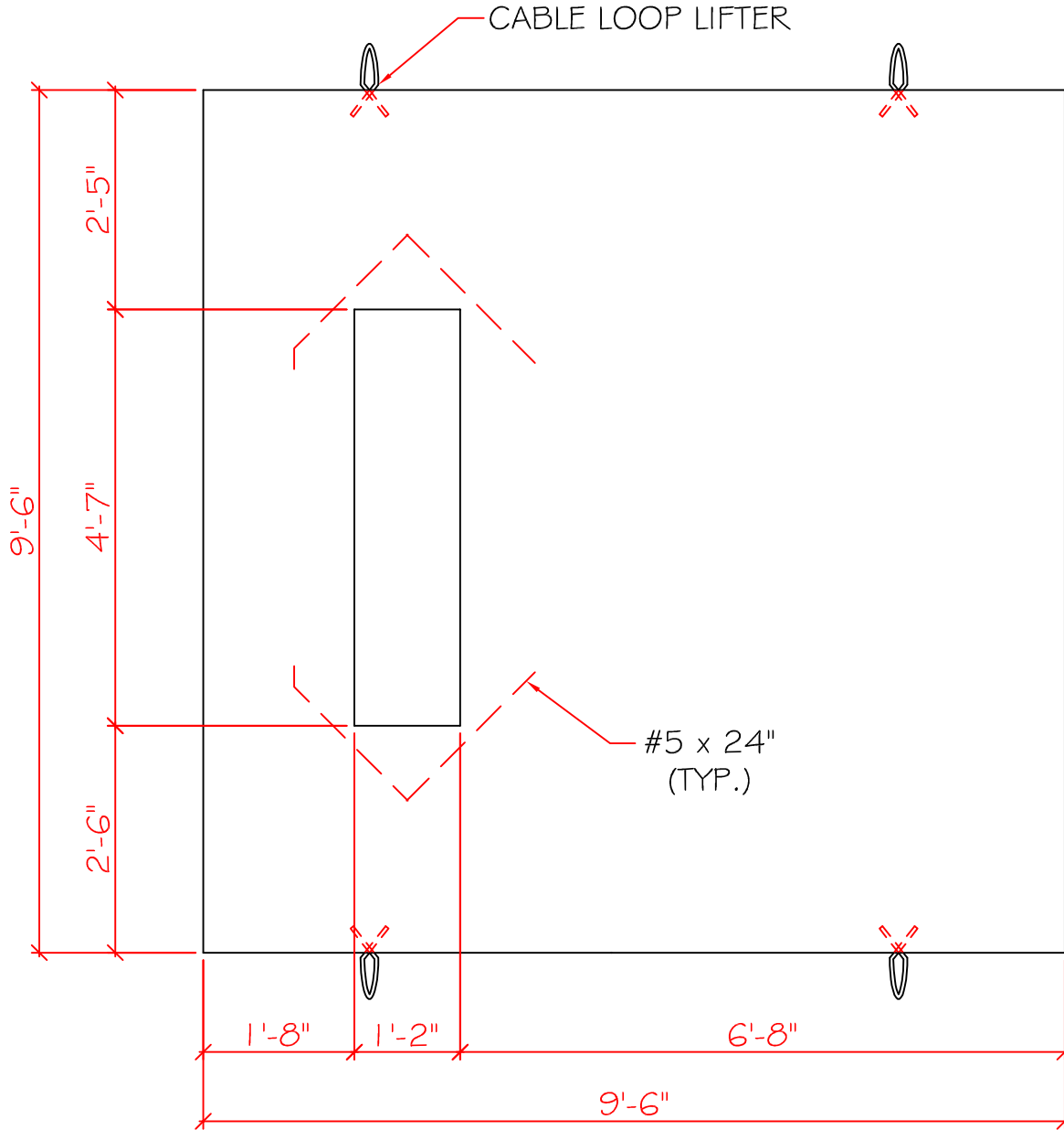
PLAN VIEW
