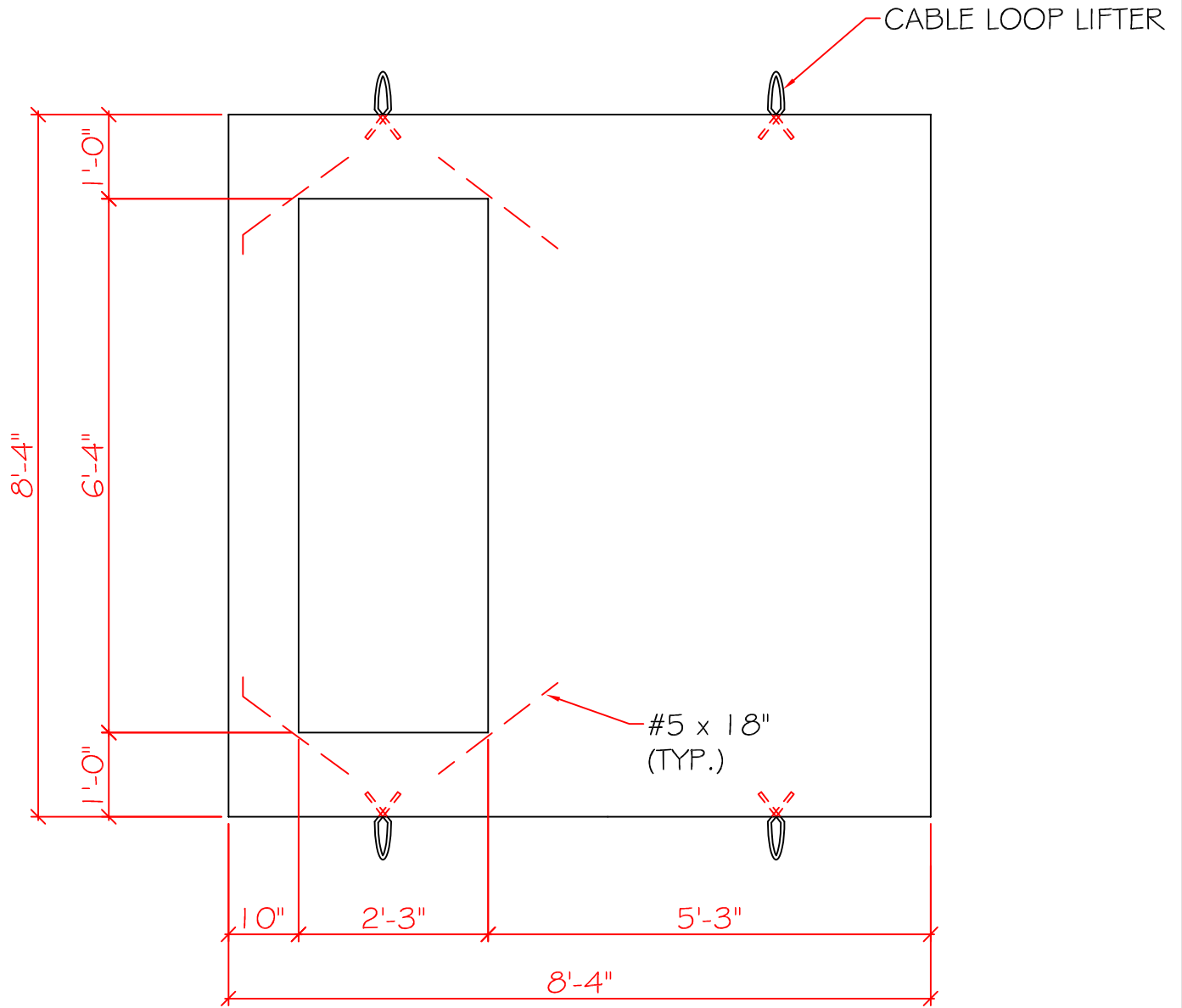
PLAN VIEW
