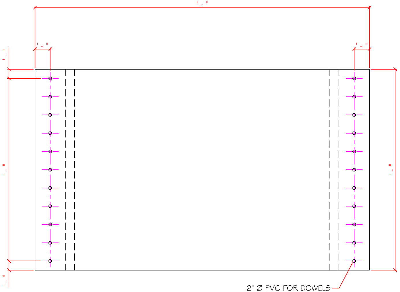
PLAN VIEW
